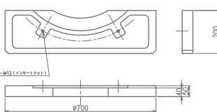
11 S-RB50(PTK)40M12
